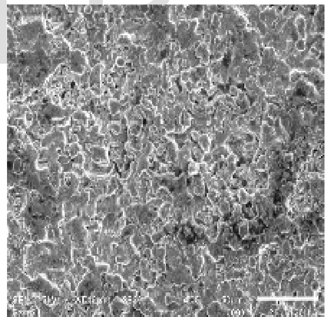
Fig. 2. Microstructure of 16Cr5Ni steel after coating with CrC-NiCr.
