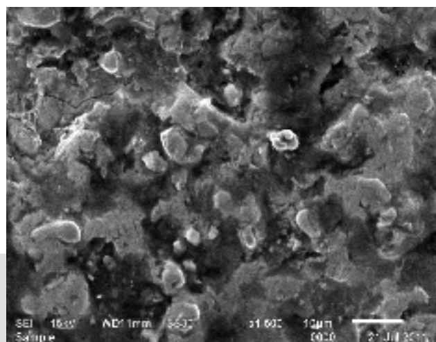
Fig.3. Specimen after conducting 2hrs erosion testing coated with CrC-NiCr
