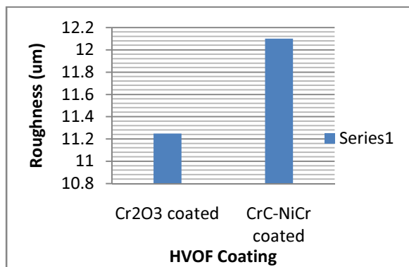
Fig.5 Roughness of coating surface 16Cr5Ni
