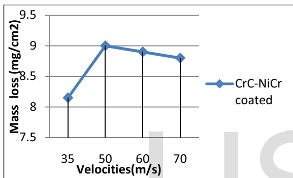
Fig. 9. Mass loss in mg/cm 2
