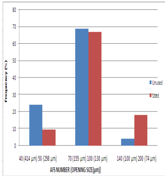
Fig. 5 Grain size distribution before and after the test in micrometers.
