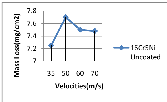
Fig. 10. Mass loss in mg/cm 2
