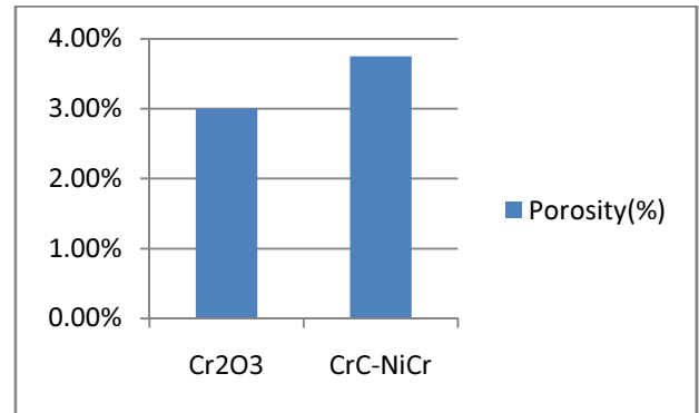
Fig.6 Porosity of coating surface 16Cr5Ni
